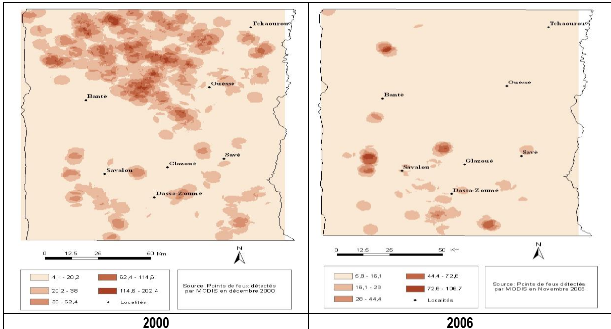
Figure 5. Fire Irradiative Power in December 2000 and November 2006
