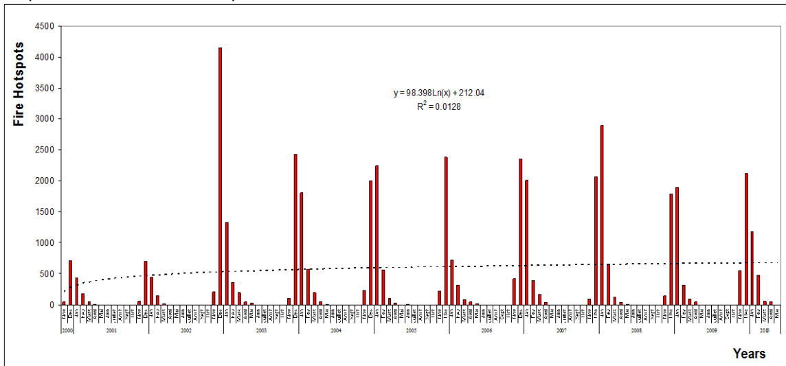
Figure 2. Figure Temporal Evolution of Fire spots from November 2000 to May 2010
