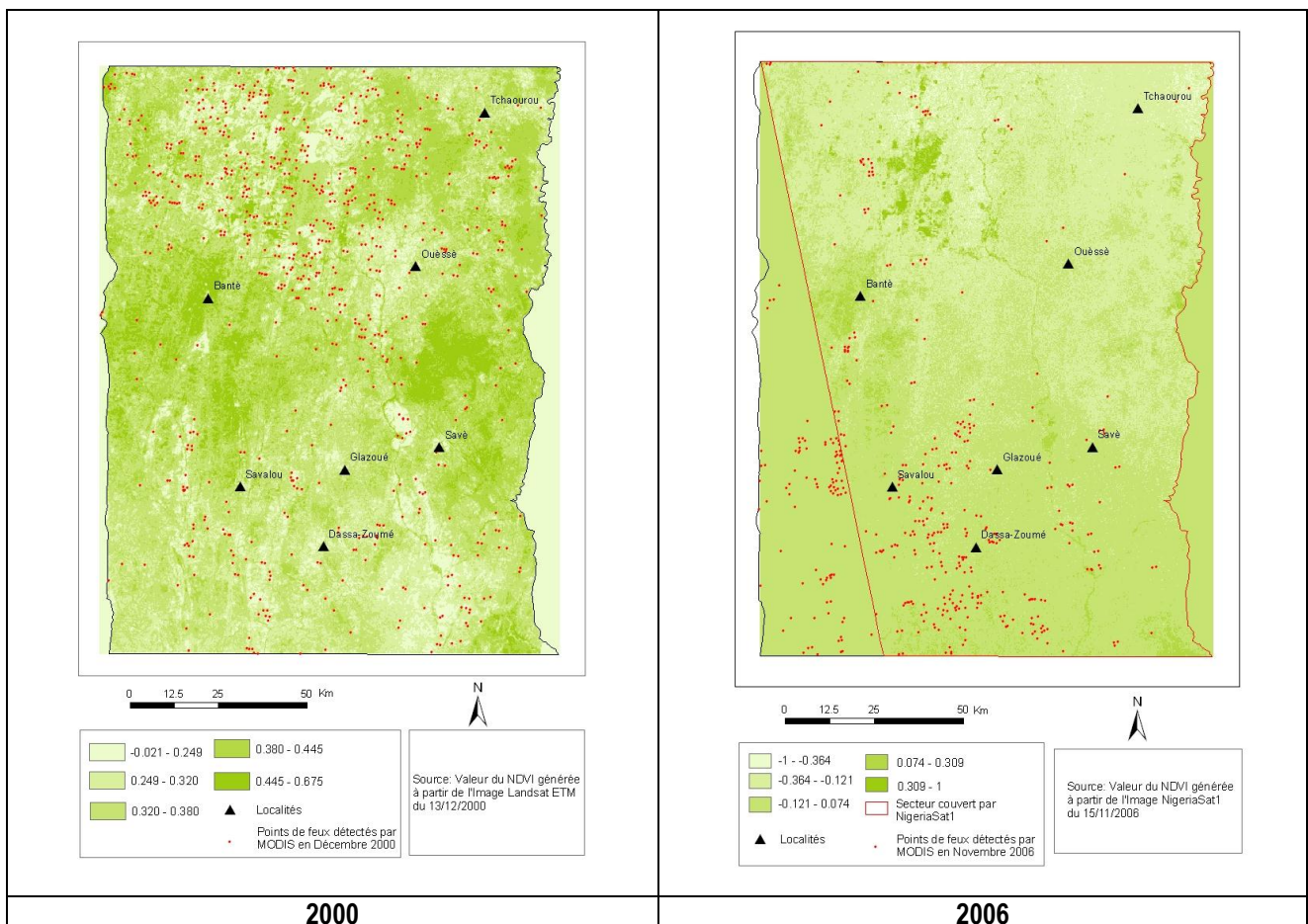
Figure 4. Normalized difference Vegetation Index (NDVI) and Hotspots Fires
